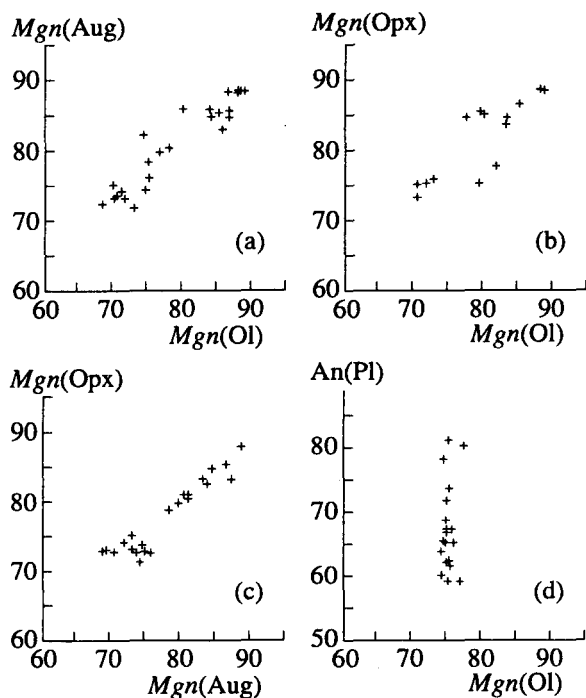
Fig. 1. Relationship between compositions of solid phase inclusion and host mineral in the aluminous basalts of the Zavaritskii outburst: (a) olivine inclusions in clinopyroxene and clinopyroxene inclusions in olivine (Aug is high-calcium pyroxene); (b) orthopyroxene inclusions in olivine; (c) orthopyroxene inclusions in clinopyroxene; (d) olivine inclusions in plagioclase. Mgn = 100Mg/(Mg + Fe^{2+}) , An = Ca/(Ca + Na + K) .
